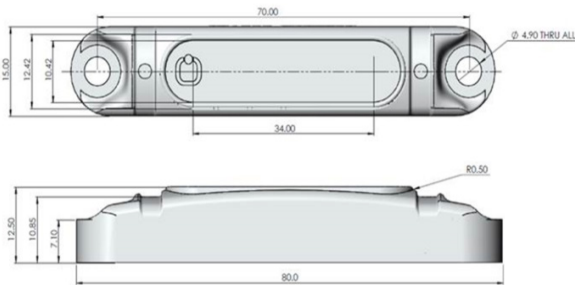
Dimensions stated in mm
